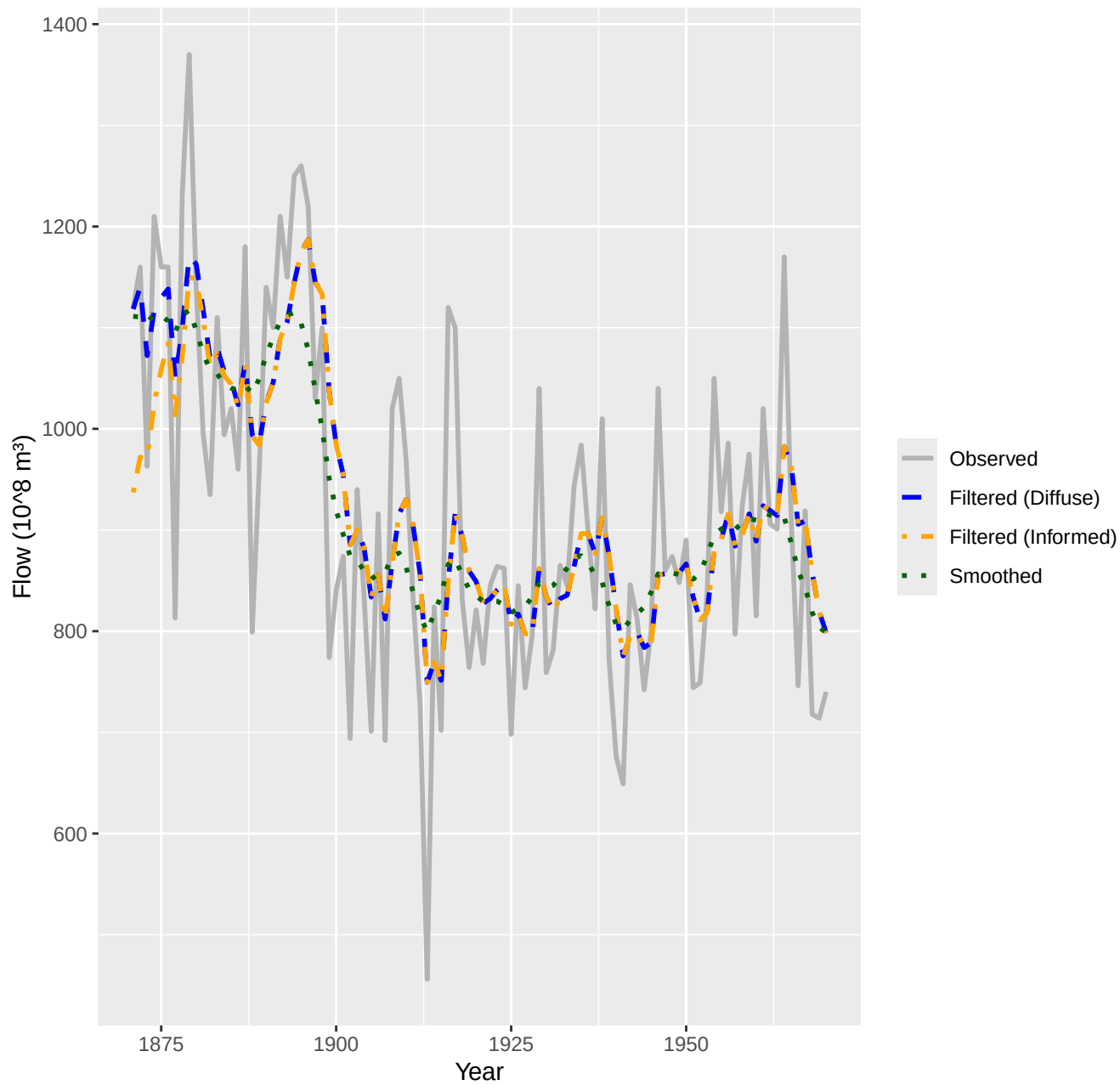
Nile River Flow: Kalman Filtering and Smoothing
